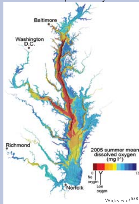
Climate change is likely to expand and intensify “dead zones,” areas where bottom water is depleted of dissolved oxygen because of nitrogen pollution, threatening living things.
