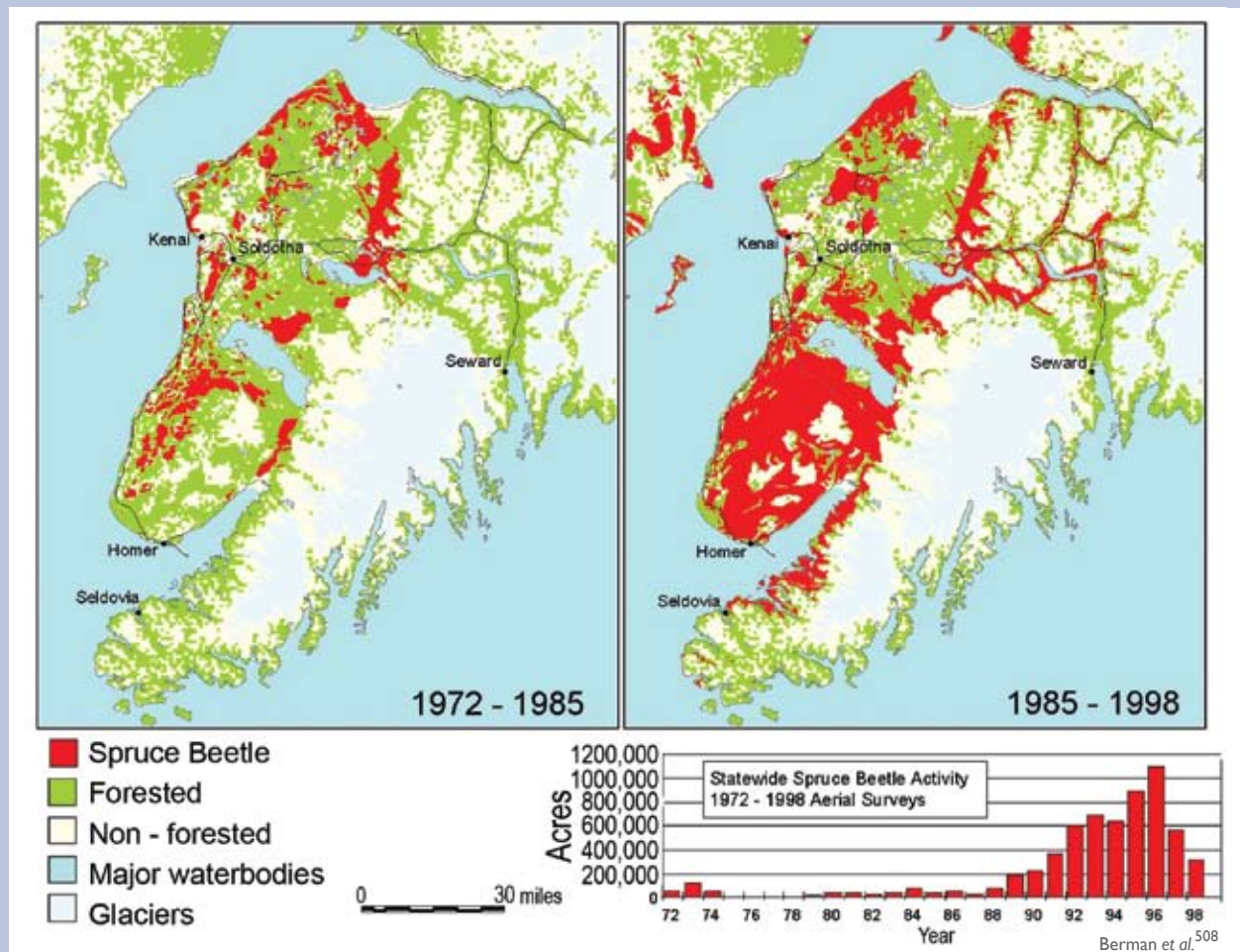
Warming in Alaska has caused insect outbreaks to increase. Red areas indicate spruce beetle infestations on the Kenai Peninsula. Over 5 million acres of Alaska spruce forests were destroyed.
