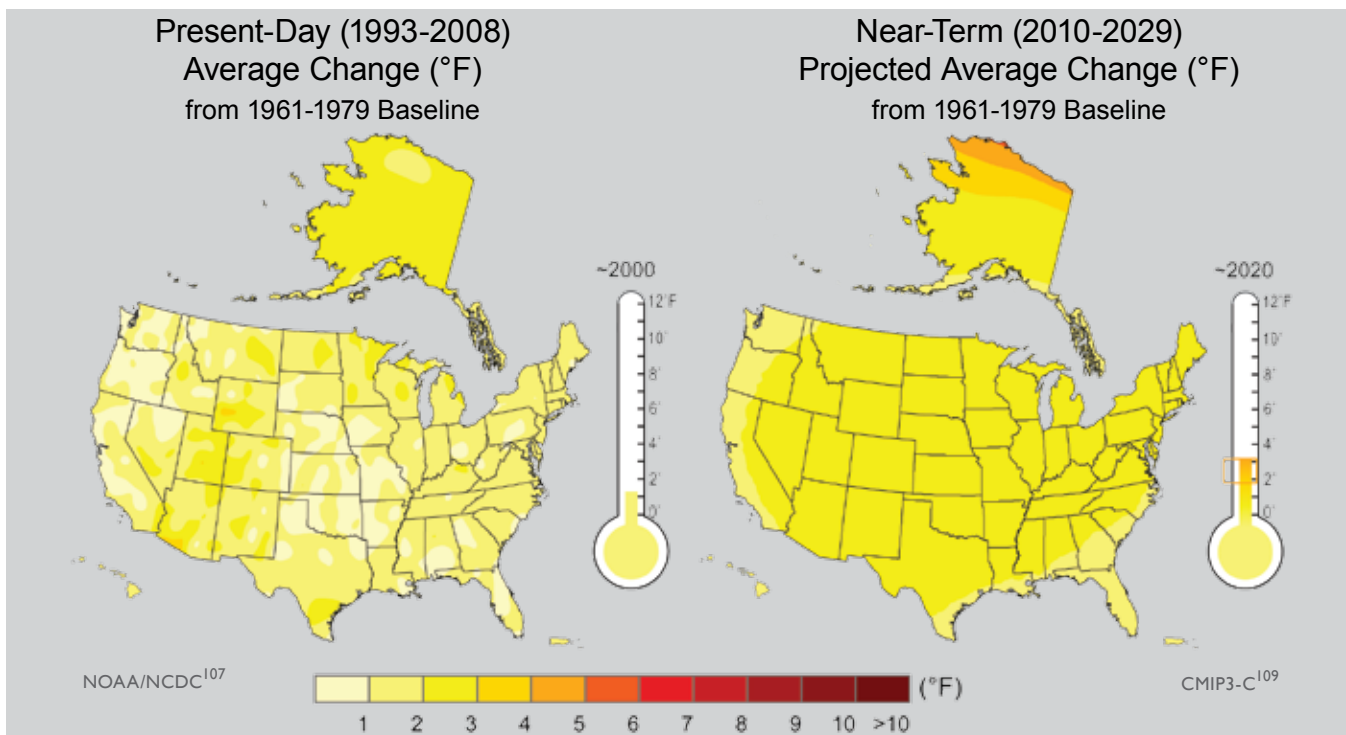
The maps and thermometers on this page and the next page show temperature differences (either measured or projected) from conditions as they existed during the period from 1961-1979. Comparisons to this period are made because the influence on climate from increasing greenhouse gas emissions has been greatest during the past five decades. The present-day map is based on the average observed temperatures from 1993-2008 minus the average from 1961-1979. Projected temperatures are based on results from 16 climate models for the periods 2010-2029, 2040-2059, and 2080-2099. The brackets on the thermometers represent the likely range of model projections, though lower or higher outcomes are possible. The mid-century and end-of-century maps show projections for both the higher and lower emission scenarios. 91 The projection for the near-term is the average of the higher and lower emission scenarios 91 because there is little difference in that timeframe.
