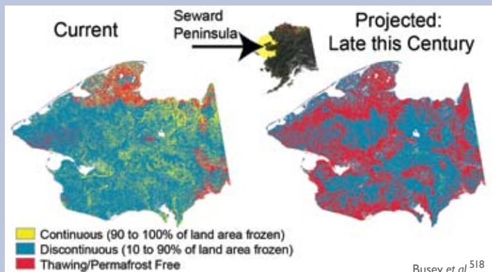
The maps show projected thawing on the Seward Peninsula by the end of this century under a moderate warming scenario approximately half-way between the lower and higher emissions scenarios 91 described on page 23.
