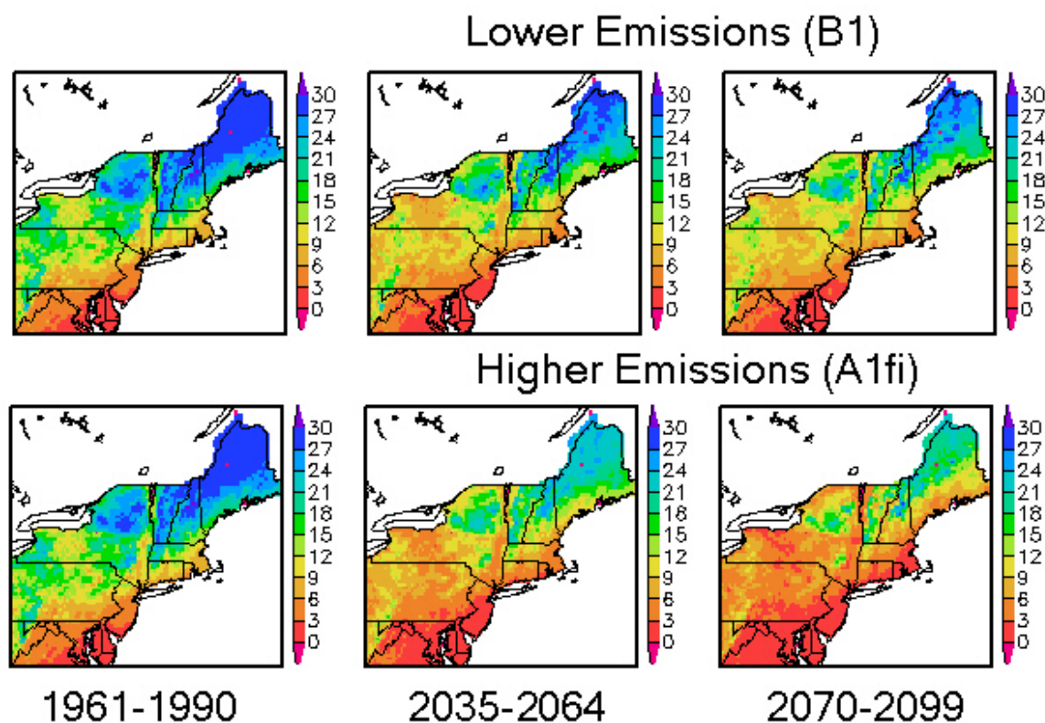
Figure 11. The number of snow-covered days per month (December–February) in the Northeast, averaged over 30-year periods. Values are the averages of the HadCM3 and PCM simulations from the VIC model.
