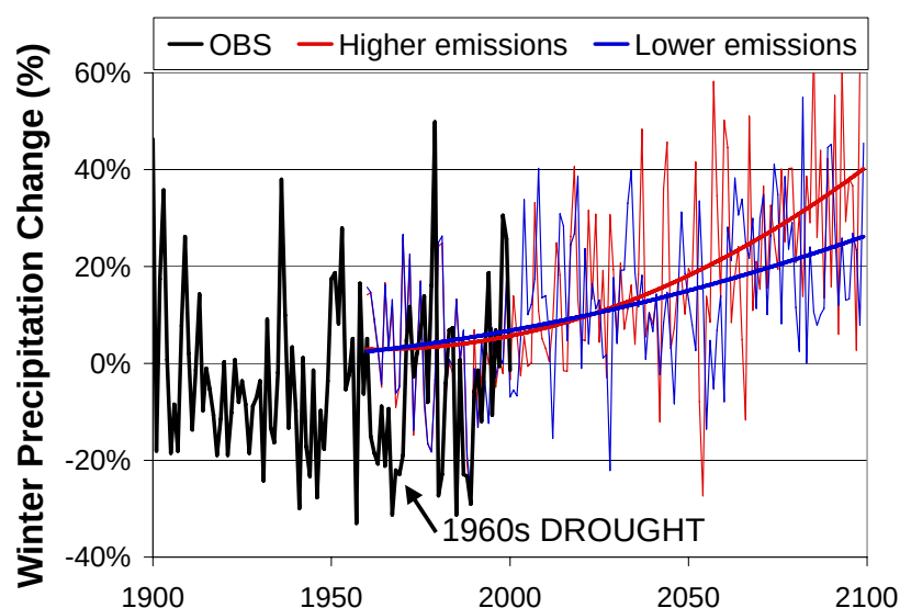
Figure 6. Observed and model-based winter precipitation for the Northeast, in units of percentage change relative to the 1961-1990 average.
