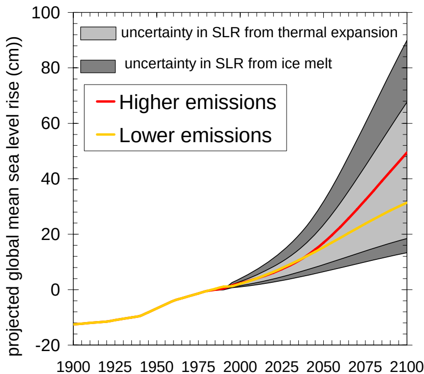
Figure 13. Model-simulated sea-level rise (SLR) under the higher- and lower-emissions scenarios. 90
